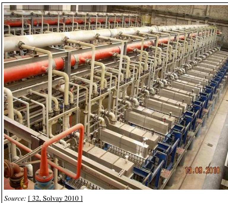
Figure 2.11: View of a membrane cell room equipped with monopolar electrolysers
